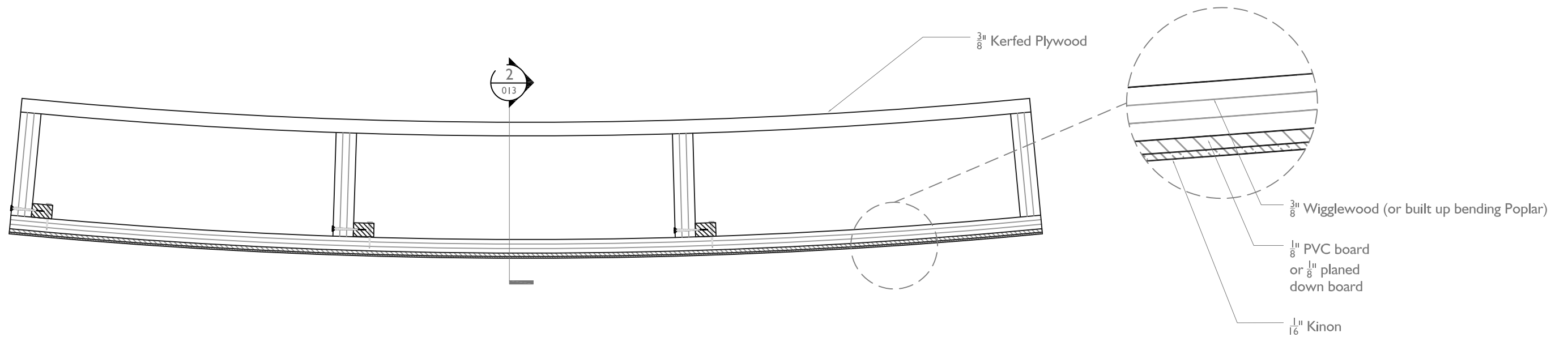
1 HORIZONTAL SECTION - PVC CONSTRUCTION 012 SCALE: 1:4
