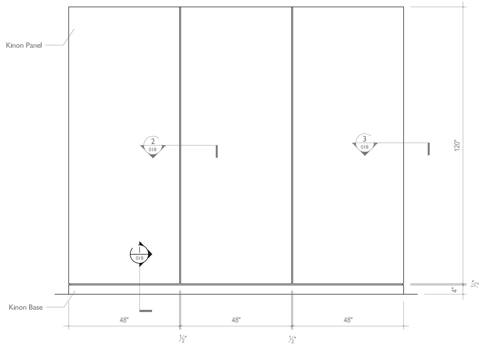
1 FRONT ELEVATION 017 SCALE: Not to scale
