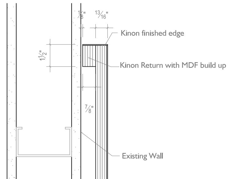
3 HORIZONTAL SECTION @ KINON WALL PANELS 08 SCALE: 3" = 1'-0"
