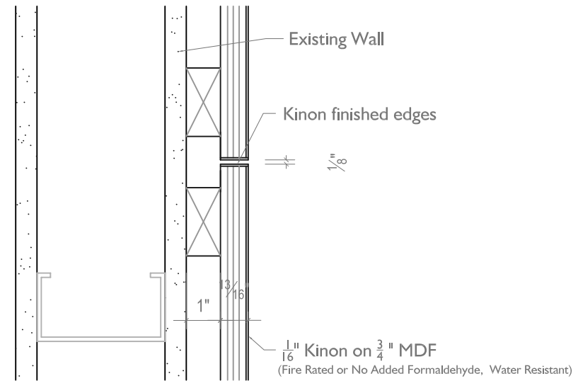
2 HORIZONTAL SECTION @ KINON WALL PANELS 08 SCALE: 3" = 1'-0"
