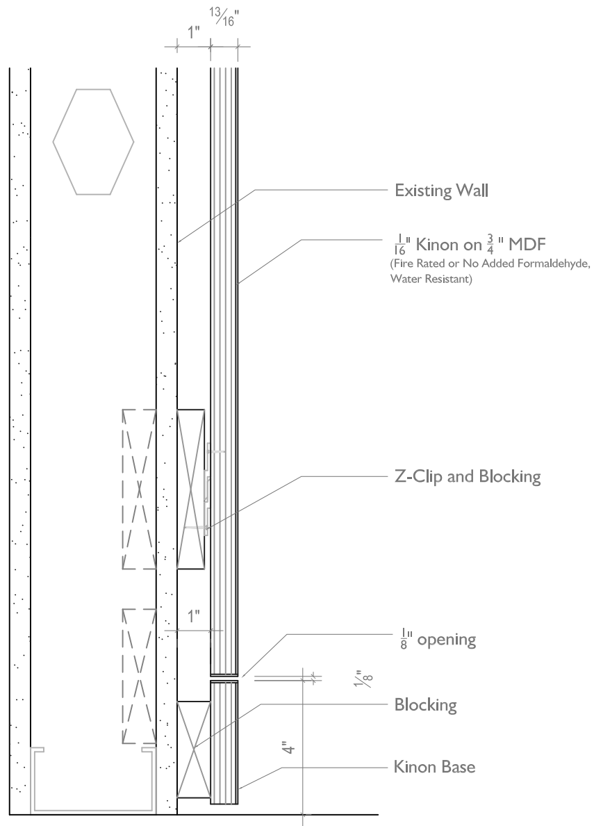
1 VERTICAL SECTION @ KINON WALL PANEL JOINT 08 SCALE: 3" = 1'-0"
