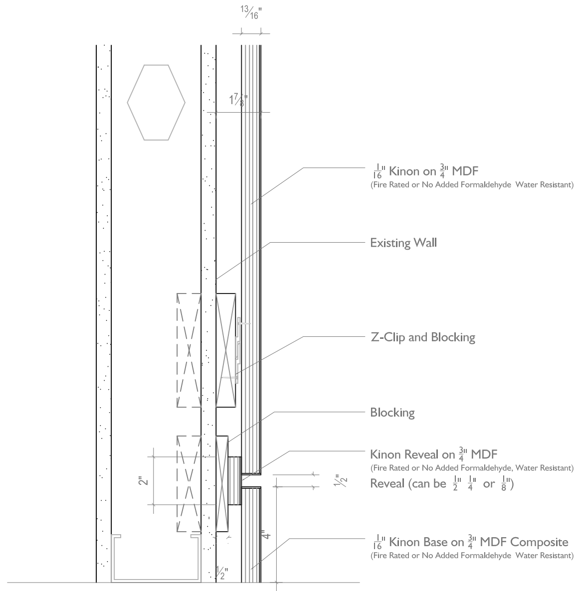
1 VERTICAL SECTION @ BASE OF KINON WALL PANELS 07 SCALE: 3"=1'-0"
