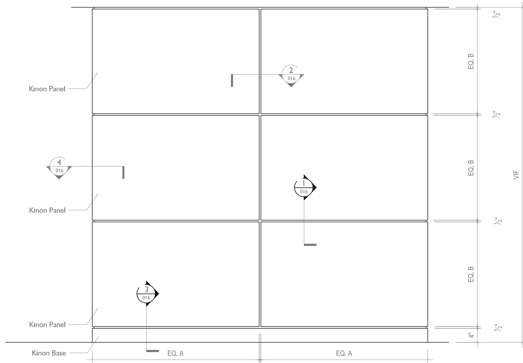
4 FRONT ELEVATION @ KINON WALL PANELS SCALE: 3/4" = 1' 0"
