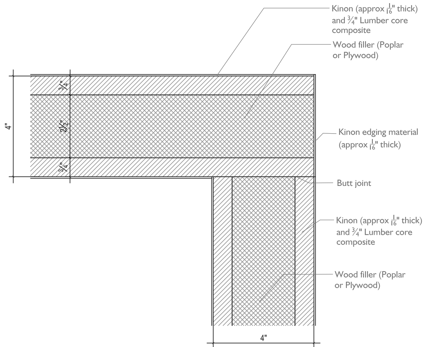
1 PARSONS TABLE - BUTT JOINT DETAIL 017 SCALE: Not to scale
