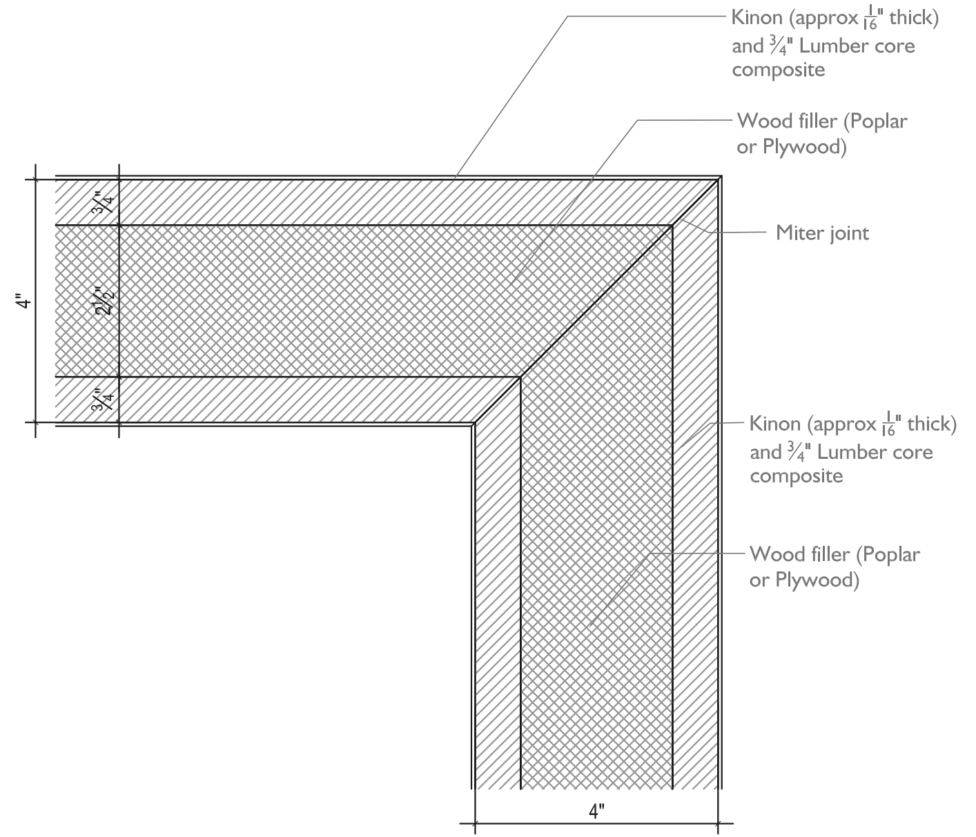
3 PARSONS TABLE - MITER JOINT DETAIL 017 SCALE: Not to scale
